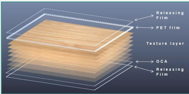
适贴盖板表面 Conformable Cover Glass Surface
